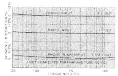
Fig. 9. Harmonic-distortion percentage.
